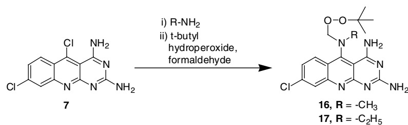
Scheme 4. Synthesis of compounds 16 and 17.
